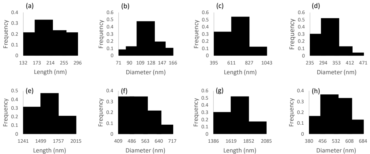
Figure 61: length and diameter distribution for NWs formed at fixed (a,b) E_{max}=130 \text{ mJ/cm}^2 , (c,d) E_{max}=175 \text{ mJ/cm}^2 , (e,f) E_{max}=215 \text{ mJ/cm}^2 , and (g,h) E_{max}=260 \text{ mJ/cm}^2 , respectively.
