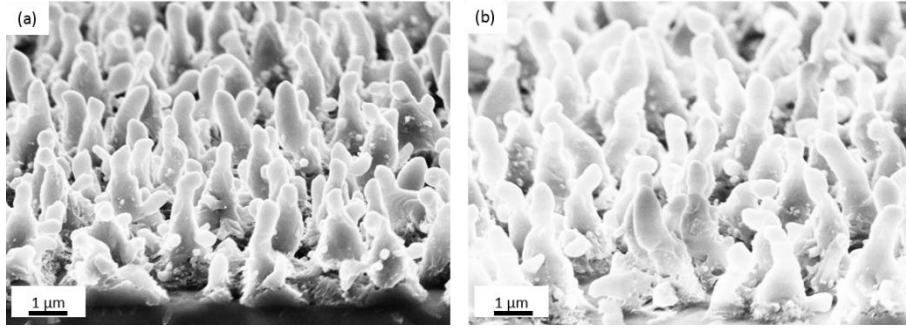
Figure 60: SEM images of Silicon NWs formed with energy density equals (a) 300 \text{ mJ/cm}^2 , and (b) 350 \text{ mJ/cm}^2 . All images are taken with 20^\circ tilt.
