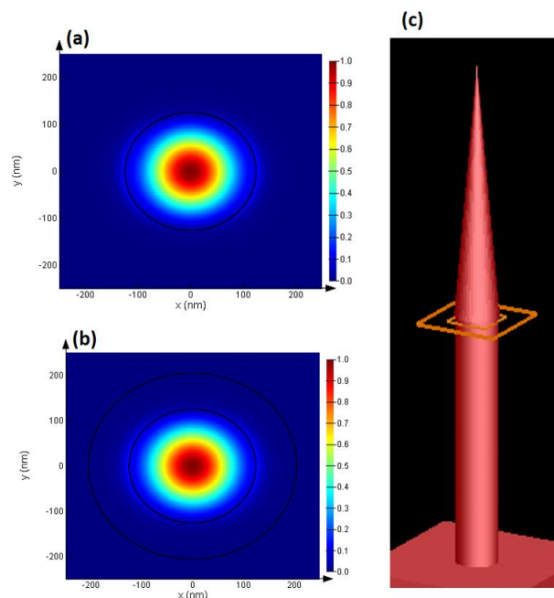
Figure 120: Fundamental mode inside TNW (a) without polymer coating and (b) with polymer coating. (c) The first location where the modes are calculated.
