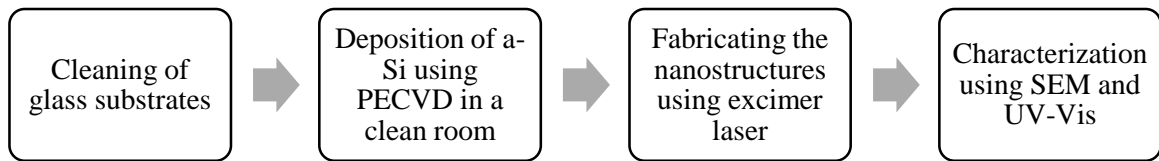
Figure 41: Fabrication process of laser annealed samples to form nanocones or nanowires.
