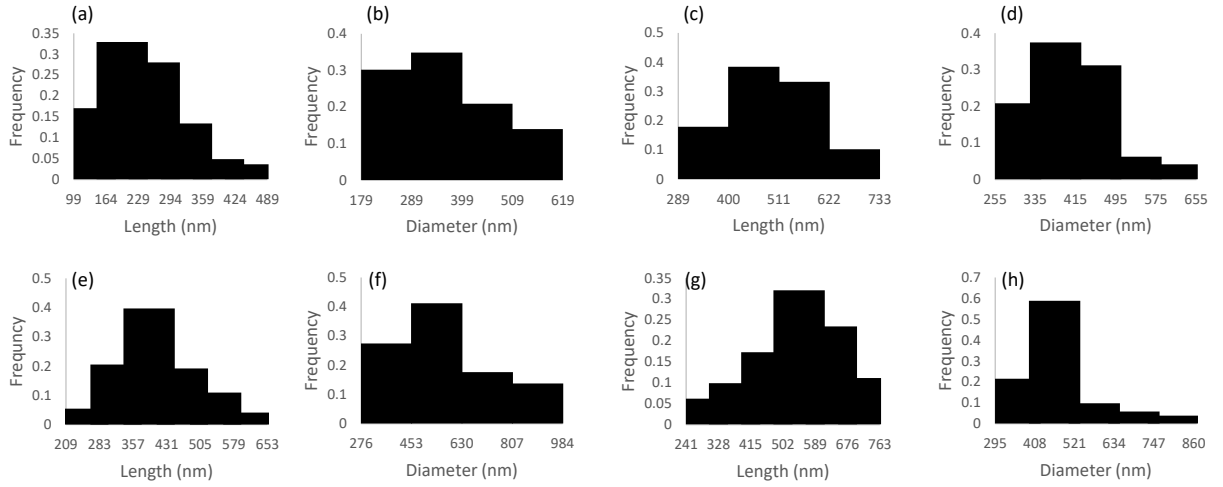
Figure 53: length and diameter distribution for for NCs formed at fixed E_{max}=300 \text{ mJ/cm}^2 and (a,b) T=20 \text{ s} , f=10 \text{ Hz} , (c,d) T=60 \text{ s} , f=10 \text{ Hz} , (e,f) T=25 \text{ s} , f=20 \text{ Hz} , and (g,h) T=25 \text{ s} , f=30 \text{ Hz} , respectively.
