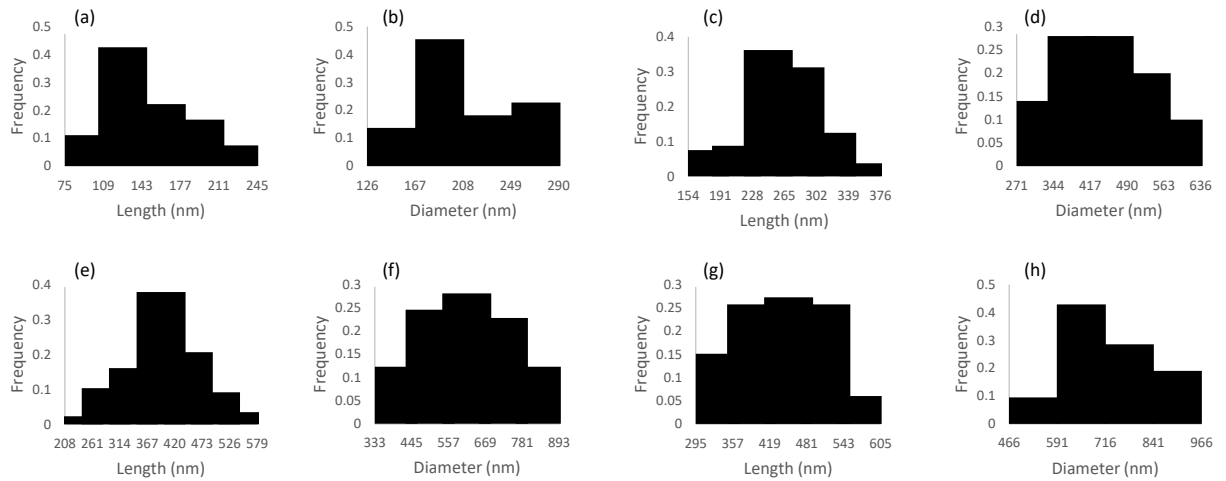
Figure 46: length and diameter distribution for the sample with (a,b) E_{max} = 215 \text{ mJ/cm}^2 , (c,d) E_{max} = 260 \text{ mJ/cm}^2 , (e,f) E_{max} = 305 \text{ mJ/cm}^2 , and (g,h) E_{max} = 345 \text{ mJ/cm}^2 , respectively.
