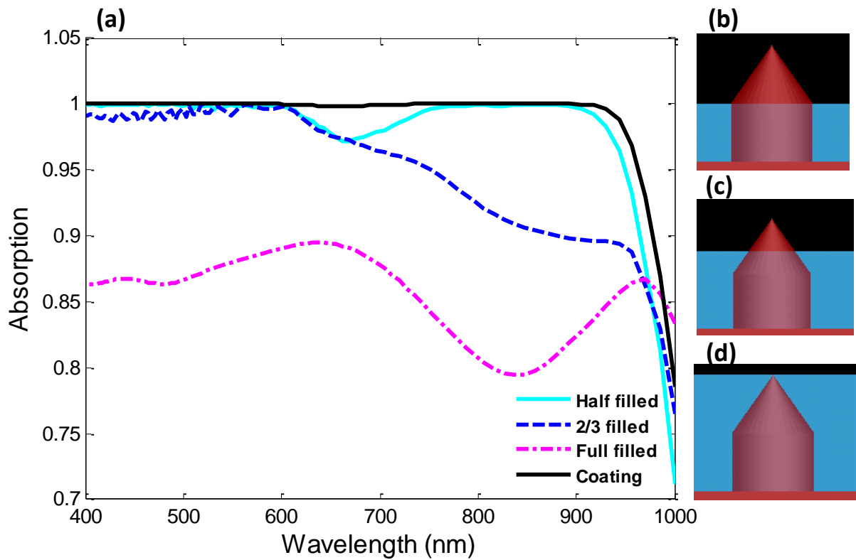
Figure 118: (a) Absorption of the optimized TNW with different polymer configurations. Schematic showing when the polymer is (b) half filled, (c) 2/3 filled, and (d) full filled.
