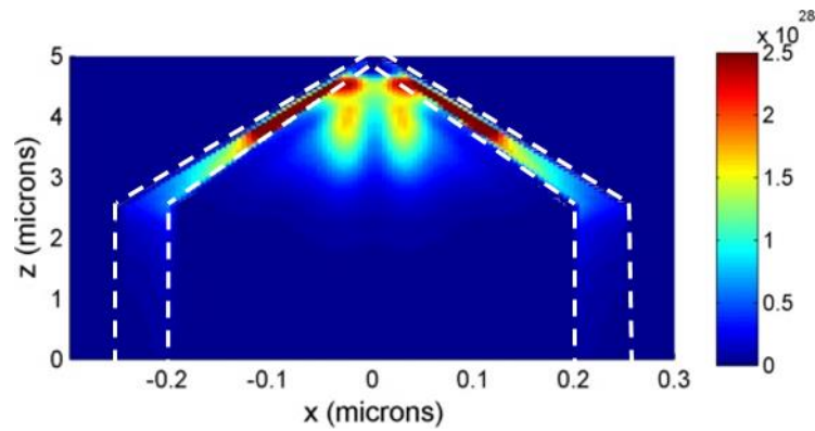
Figure 113: Generation rate inside tapered nanowires coated with PDPP3T. Units of the bar code is number of absorbed photons/m 3 s.
