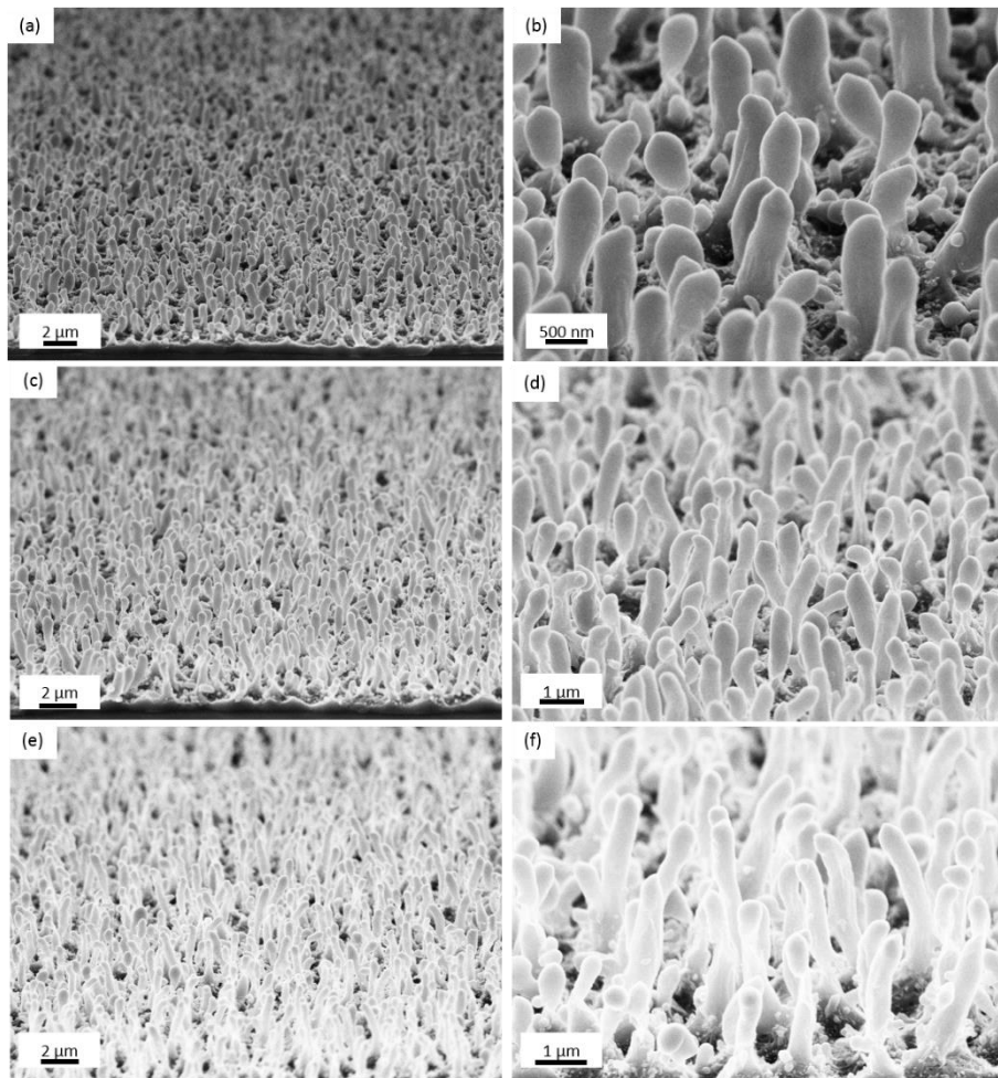
Figure 66: SEM of NWs fabricated with fixed laser energy equals 215 \text{ mJ/cm}^2 and exposure time equals 30 seconds and frequency equals (a,b) 20 Hz, (c,d) 30 Hz, and (e,f) 40 Hz. All images are taken with 20^\circ tilt.
