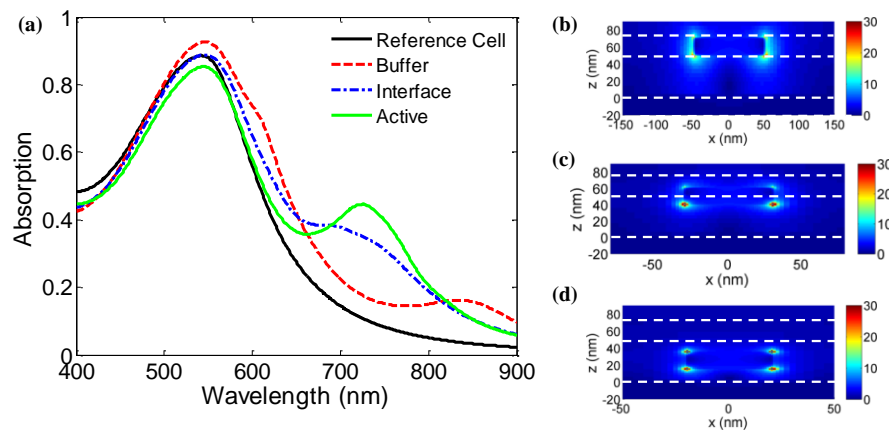
Figure 40: (a) Absorption inside P3HT:PC 70 BM for all 3 configurations for the ZrN ND. (b), (c), and (d) Electric field for ND inside the buffer layer at 850nm, at the interface at 712 nm, and inside the active layer at 720nm, respectively. Units of the bar code are V/m.
