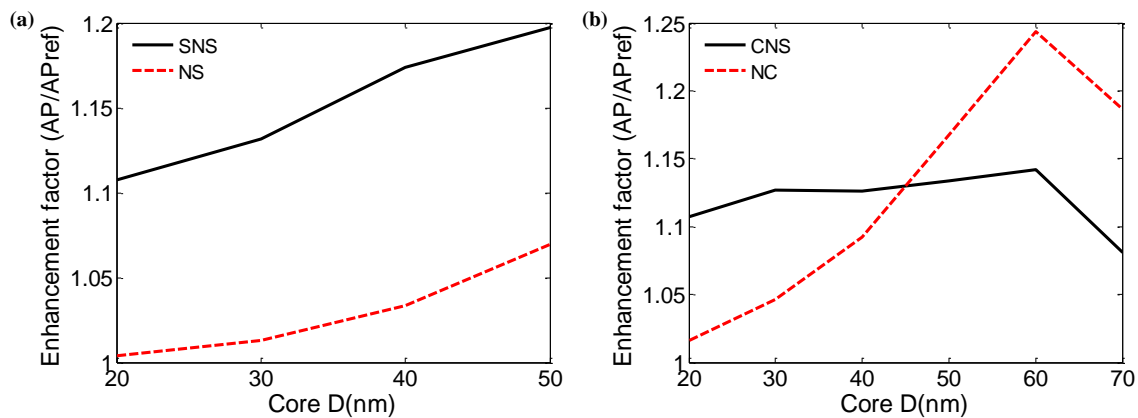
Figure 35: (a) Enhancement factor for spherical nanoshells with different core diameters and shell T = 20nm (black solid line) and for nanospheres with different diameters (red dashed line) for P = 250 nm. (b) Enhancement Factor for cubical nanoshells with different core edge lengths and shell thickness = 10nm (black solid line) and for nanocubes with different edge lengths (red dashed line) for P = 250 nm.
