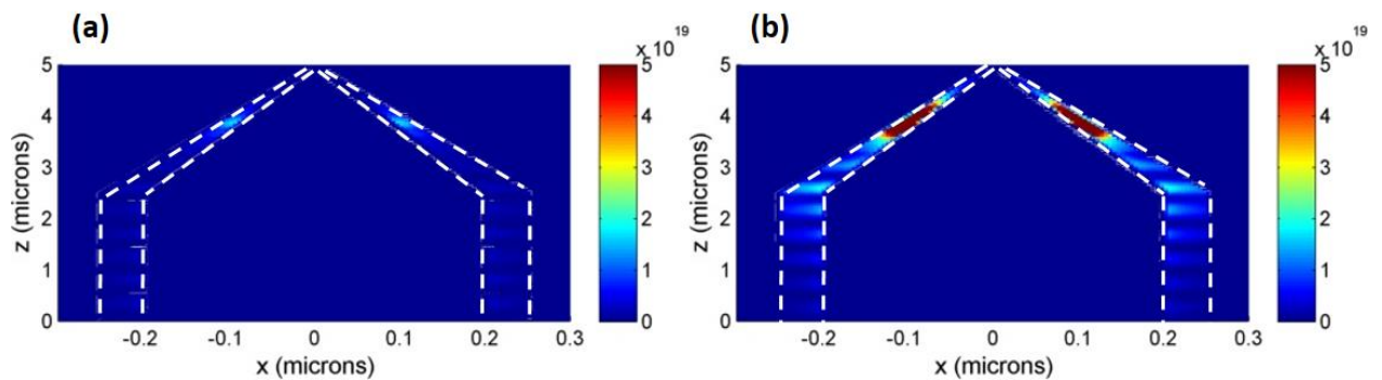
Figure 111: Absorption at 900 nm for TNW coated with (a) P3HT:PCBM and (b) PDPP3T. Units of the bar code is W/m^3 .
