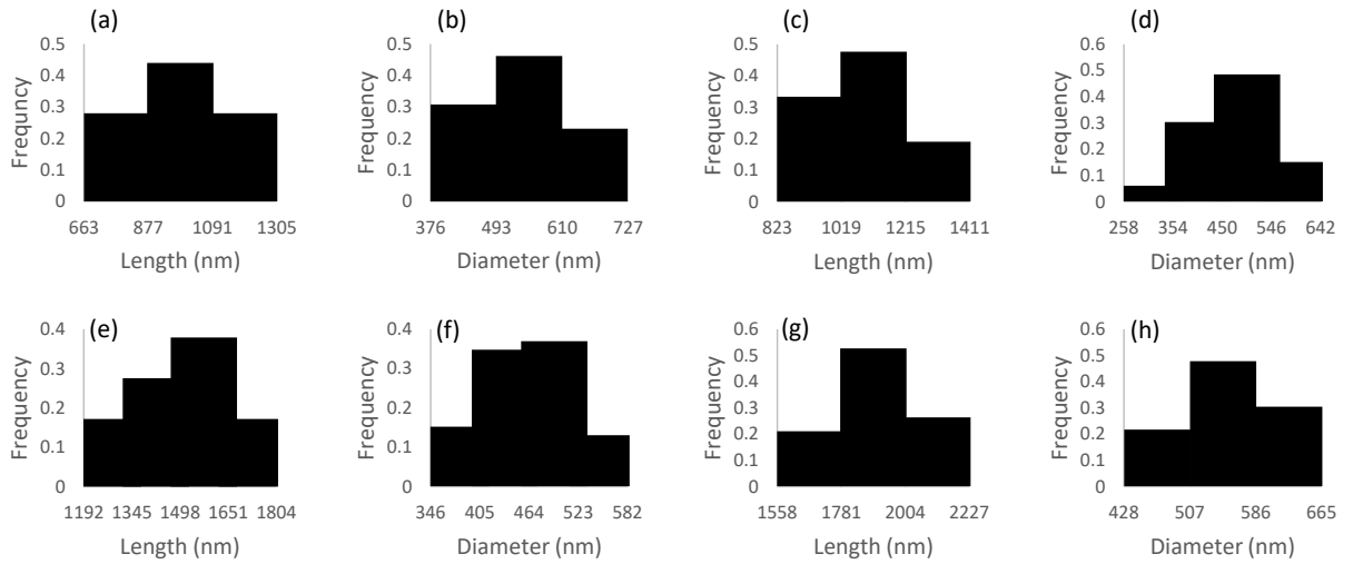
Figure 64: length and diameter distribution for NWs formed with fixed laser energy equals 215 mJ/cm 2 and frequency equals 10 Hz and time equals (a,b) 20 s, (c,d) 30 s, (e,f) 50 s, and (g,h) 60 s, respectively.
