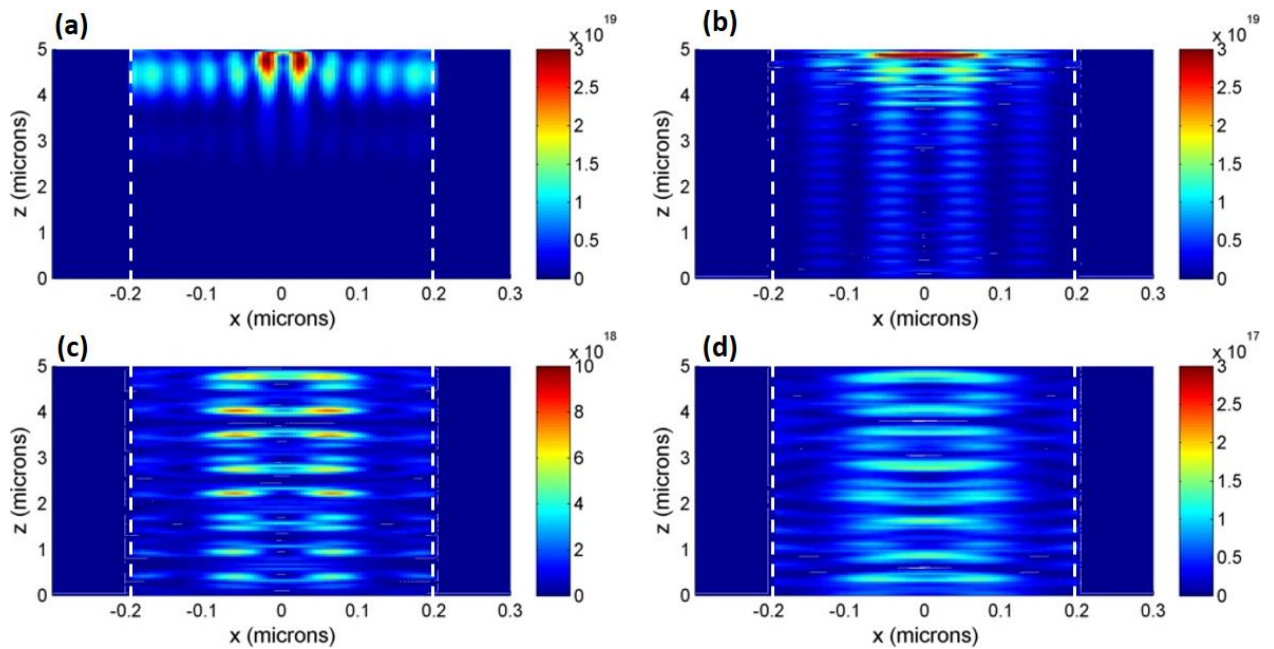
Figure 106: Absorption fields for conventional NWs at (a) 400 nm, (b) 600 nm, (c) 750 nm, and (d) 900 nm. Units of the bar code is W/m^3 .
