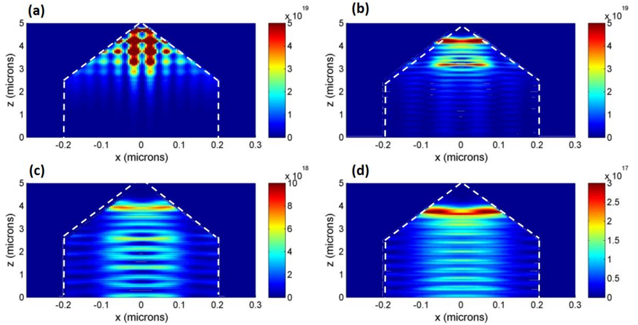
Figure 107: Absorption fields for tapered NWs at (a) 400 nm, (b) 600 nm, (c) 750 nm, and (d) 900 nm. Units of the bar code is W/m^3 .
