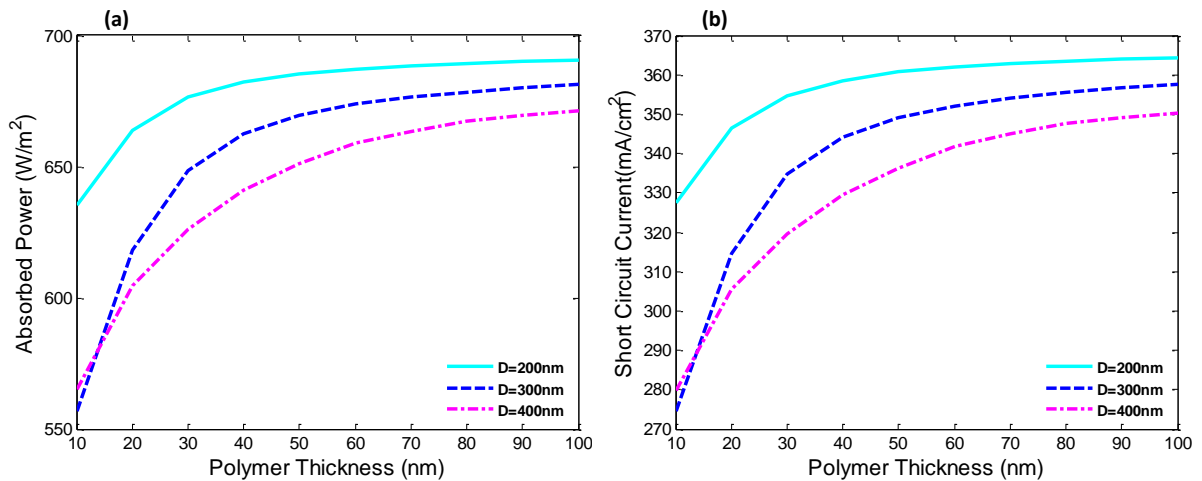
Figure 115: (a) Absorbed power and (b) short circuit current versus polymer coating thickness for several TNW diameters.
