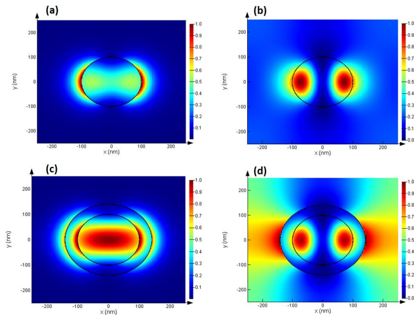
Figure 125: (a,c) The fundamental mode and (b,d) the key mode in the second location along the TNW at 900 nm with and without polymer coating, respectively.
