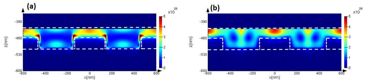
Figure 83: Generation rate for (a) solar cell with NGs for TE polarized light, and (b) solar cell with NGs for TM polarized light. Units of the bar code is number of absorbed photons/ m^3 s .
