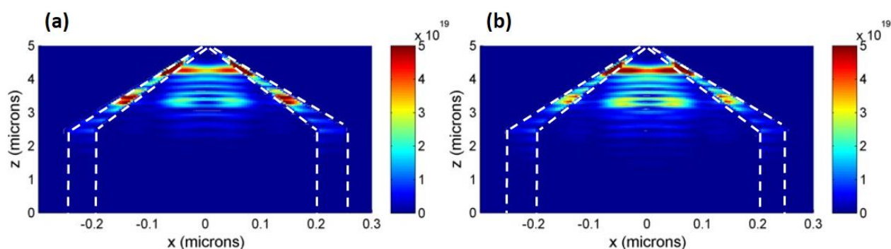
Figure 109: Absorption at 600 nm for TNW coated with (a) P3HT:PCBM and (b) PDPP3T. Units of the bar code is W/m^3 .
